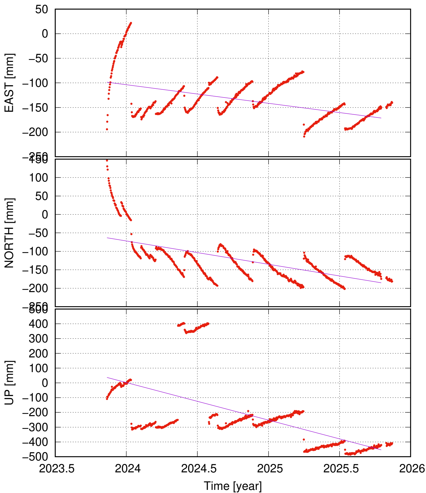
AUSV ( , ) time series (IGb20) ve = +- ; vn = +- ; vu = +- mm/yr
