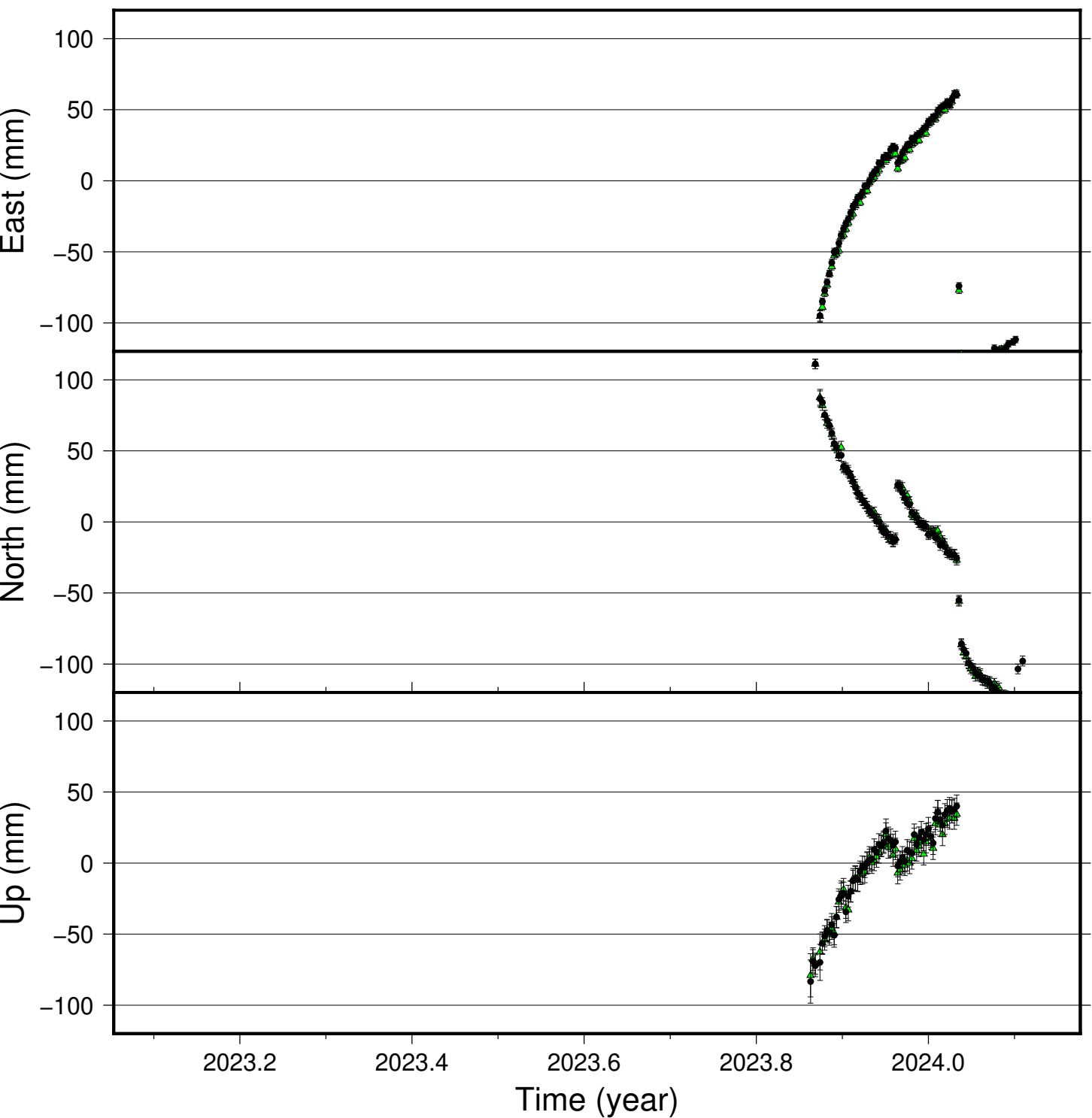
AUSV time series (IGS 2014), last 400 days
