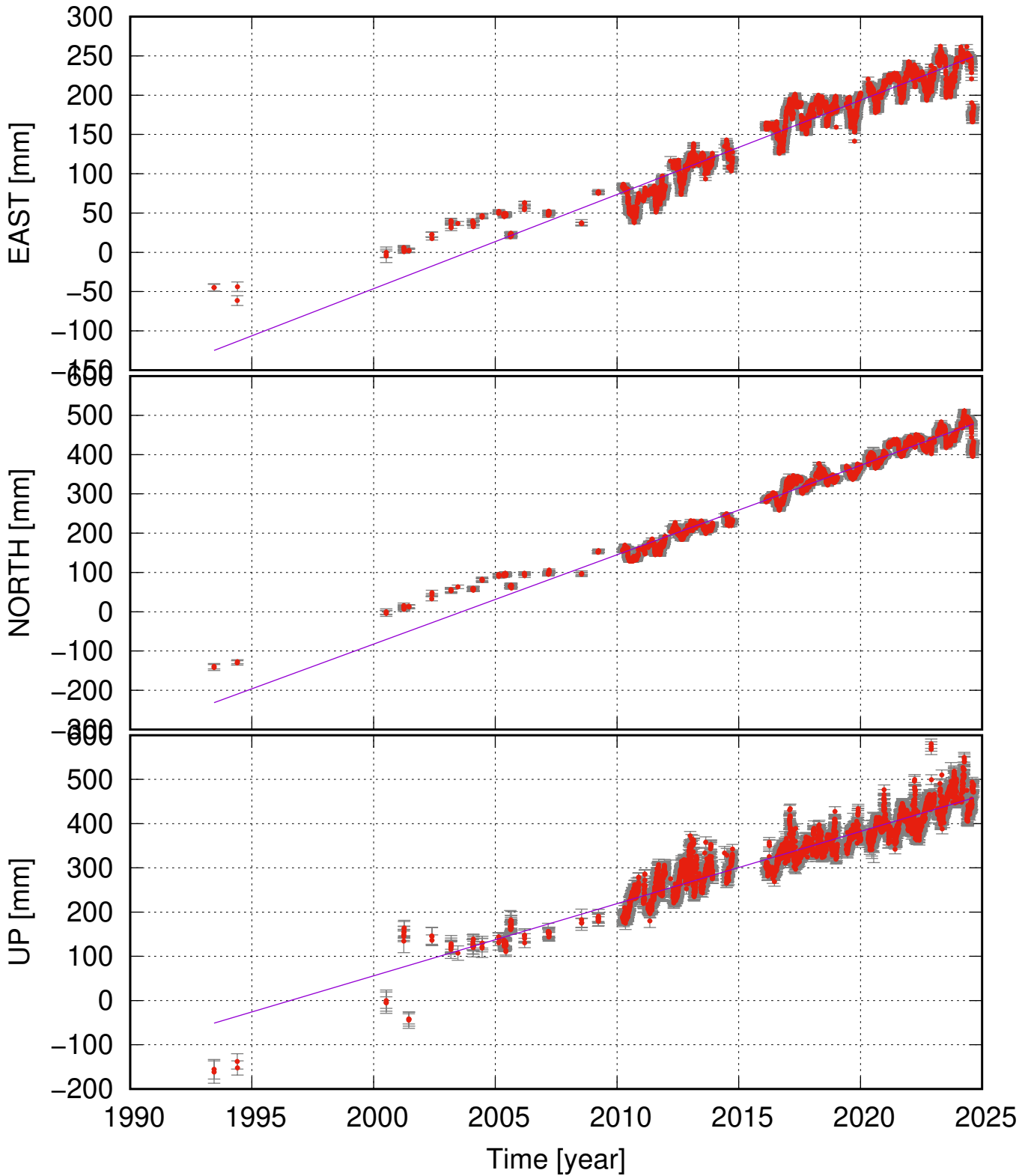
AUST (63.67, -19.08) time series (ITRF 2014) v_e = 11.98 \pm 0.55 ; v_n = 22.73 \pm 0.62 ; v_u = 16.33 \pm 0.84 mm/yr
