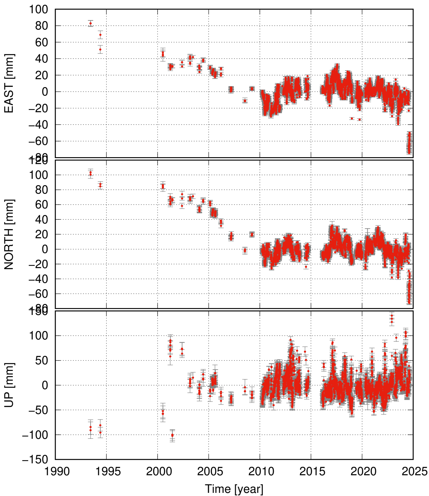
AUST detrended and seasonal signal removed
