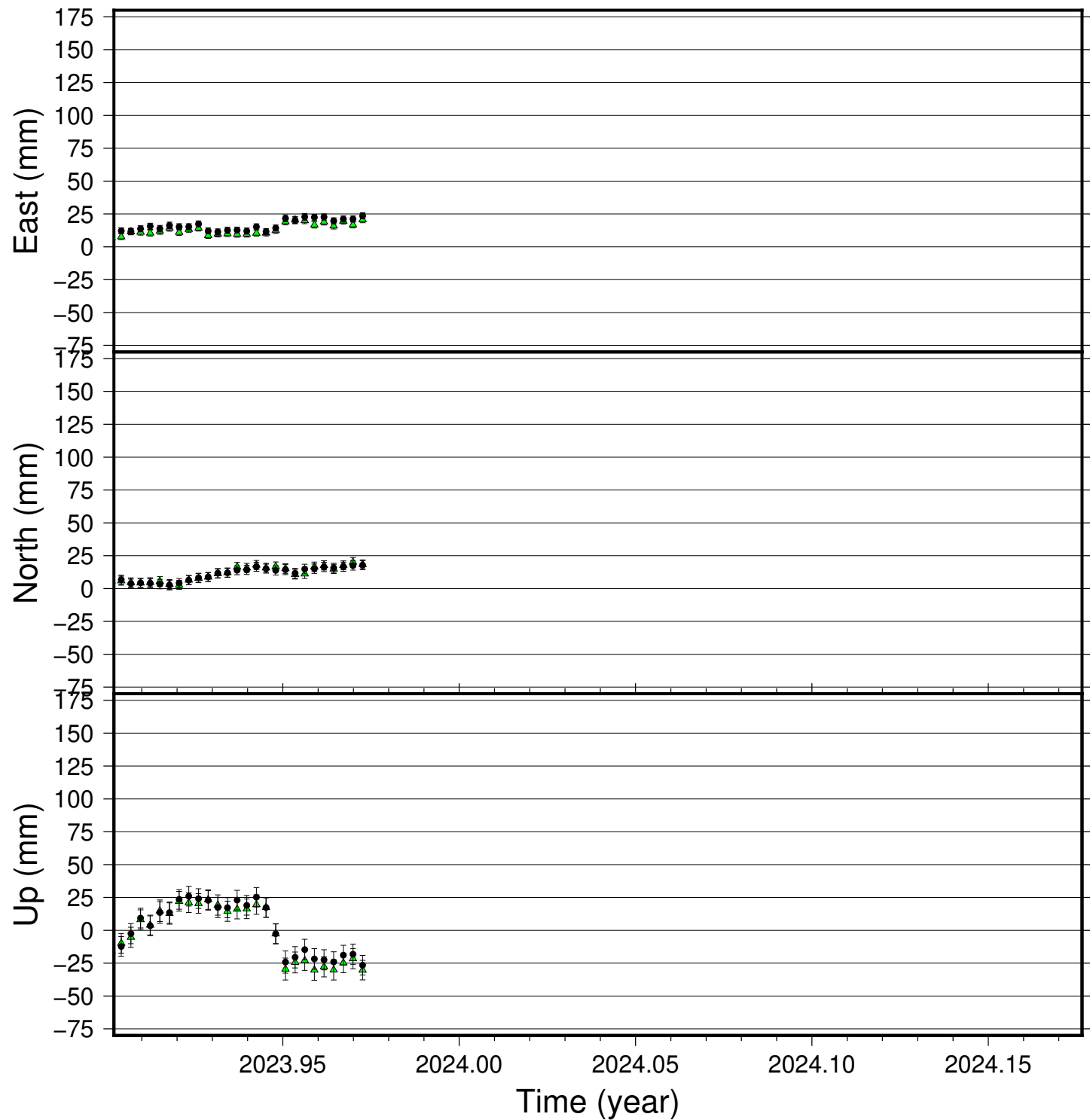
AUST time series (IGS 2014), last 100 days
