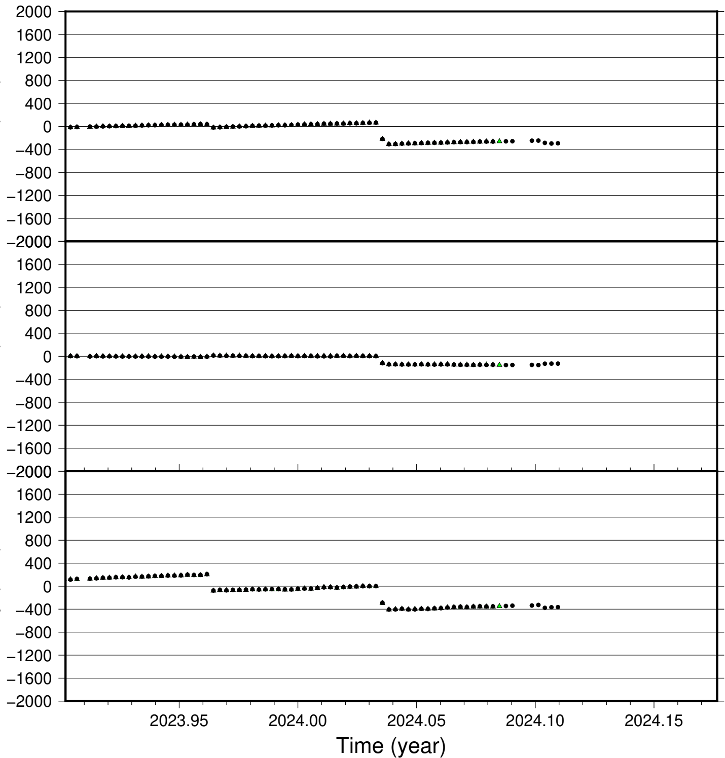
ASVE time series (IGS 2014), last 100 days
