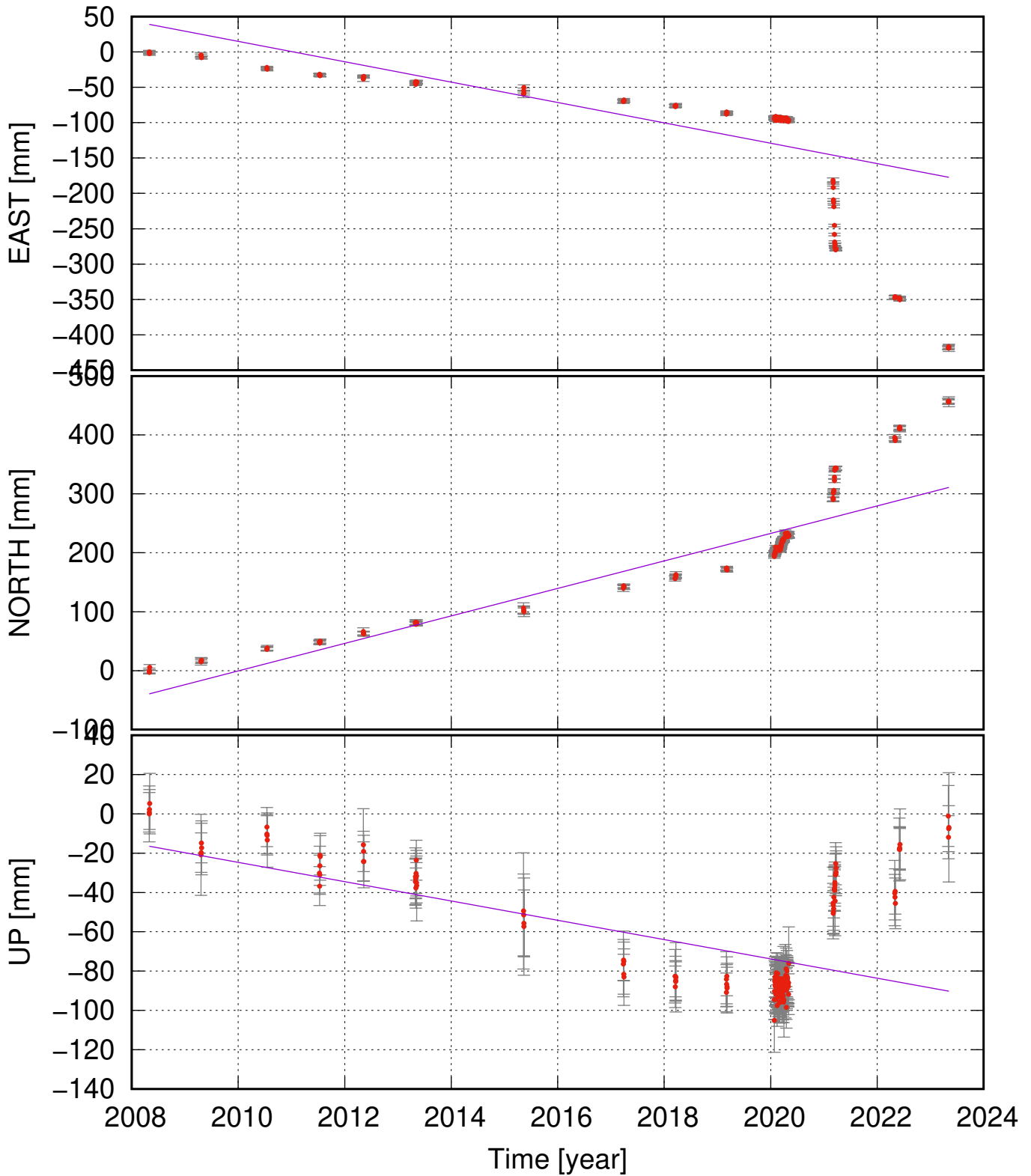
ARSE (63.91, -22.42) time series (ITRF 2014) v_e = -14.40 \pm 4.78 ; v_n = 23.31 \pm 3.09 ; v_u = -4.92 \pm 1.74 mm/yr
