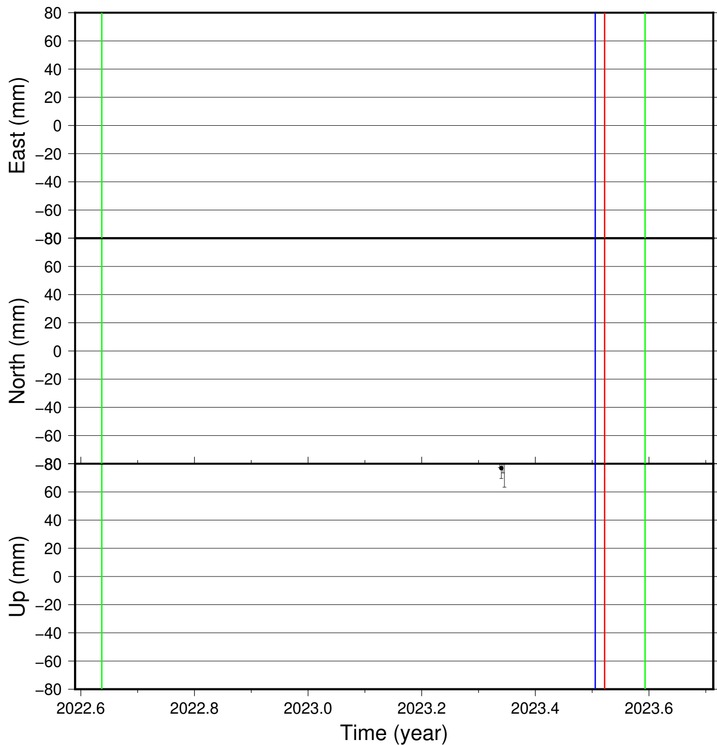
ARSE time series (IGS 2014), last 400 days
