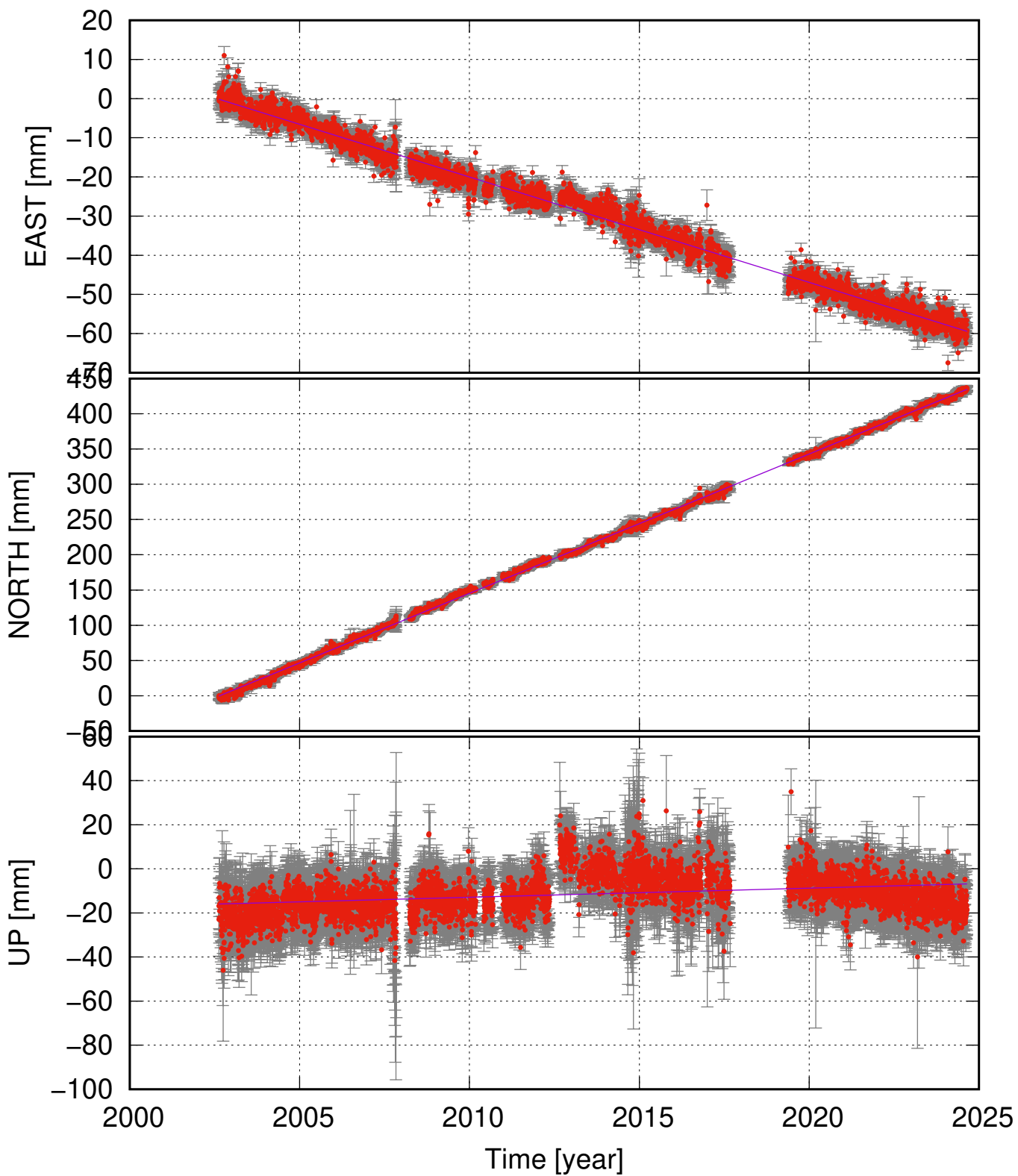
ARHO (66.19, -17.11) time series (ITRF 2014) ve = -2.69 \pm 0.08 ; vn = 19.76 \pm 0.14 ; vu = 0.41 \pm 0.36 mm/yr
