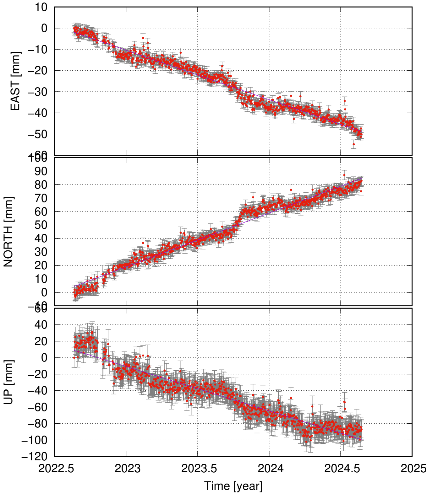
ALM9 (66.16, -19.04) time series (ITRF 2014) v_e = -23.32 \pm 1.27 ; v_n = 39.91 \pm 2.03 ; v_u = -53.86 \pm 4.72 mm/yr
