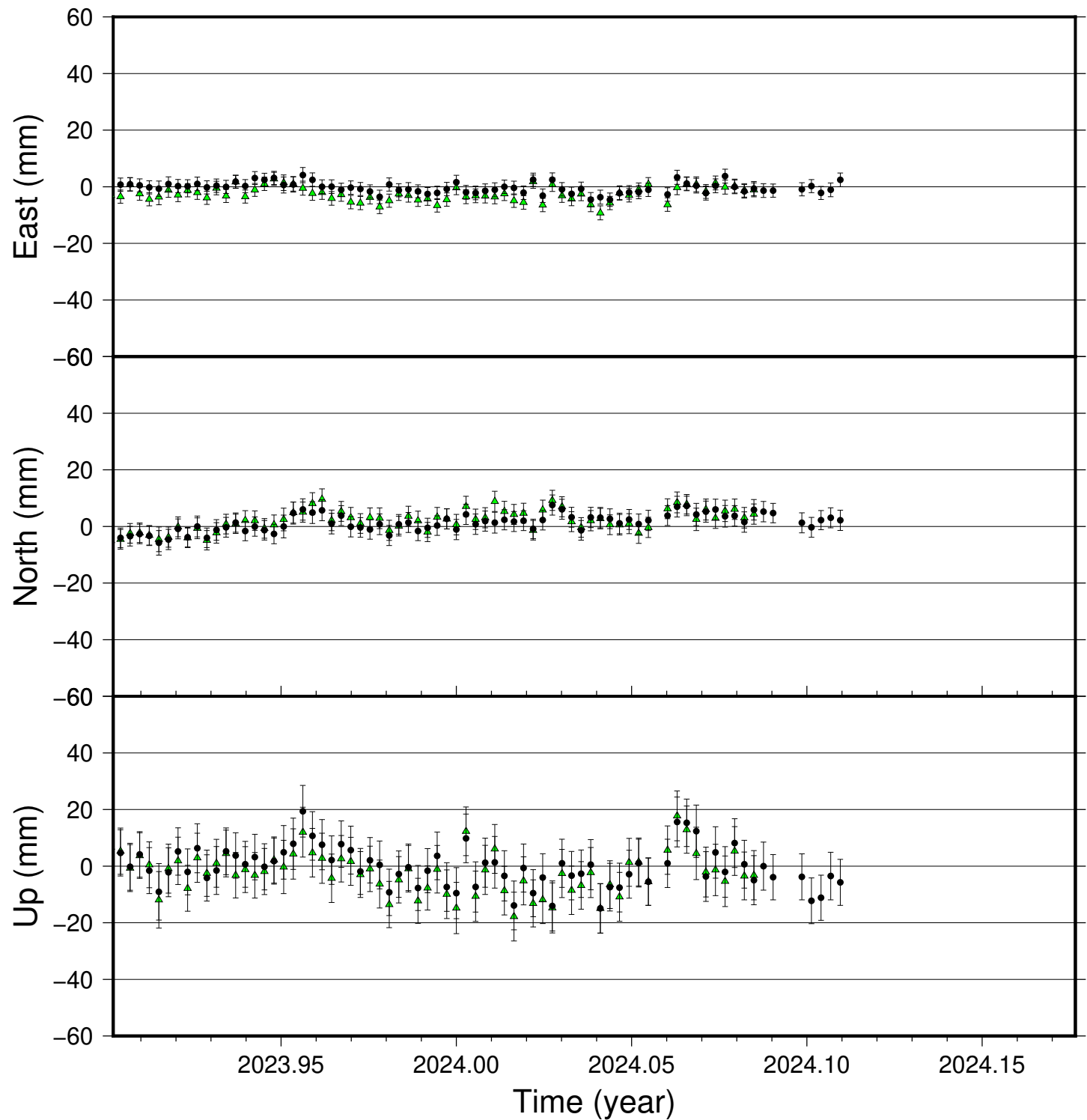
ALM9 time series (IGS 2014), last 100 days
