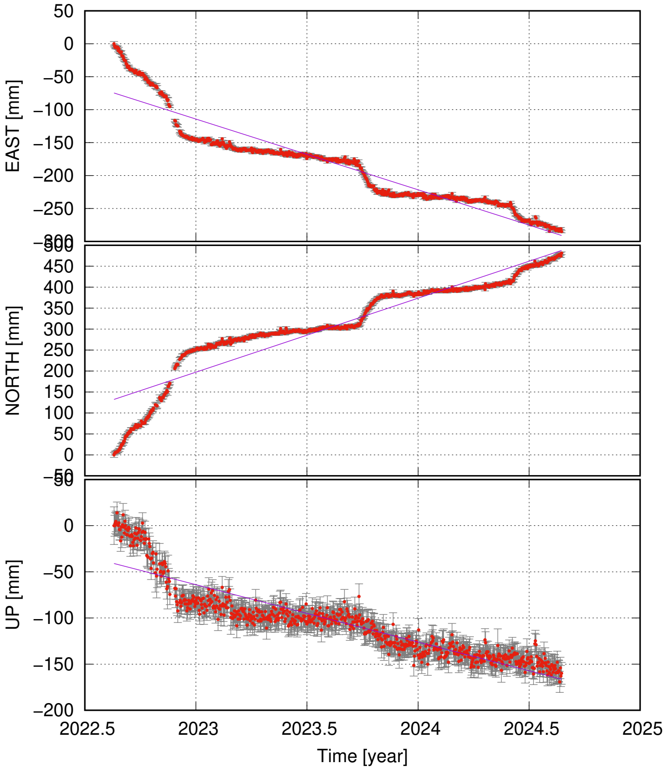
ALM8 (66.16, -19.05) time series (ITRF 2014) v_e = -107.28 \pm 10.63 ; v_n = 176.31 \pm 19.40 ; v_u = -62.17 \pm 8.02 mm/yr
