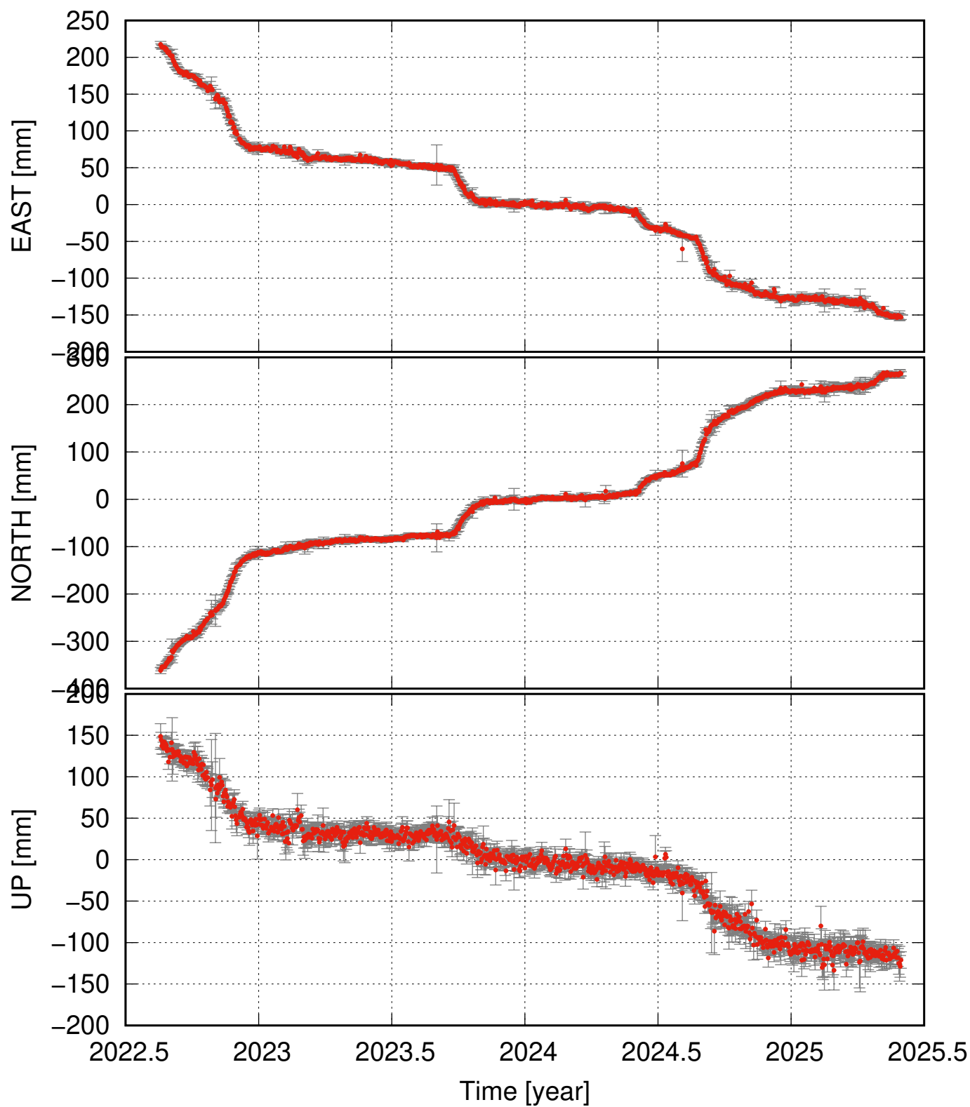
ALM8 time series relative to the NA plate
