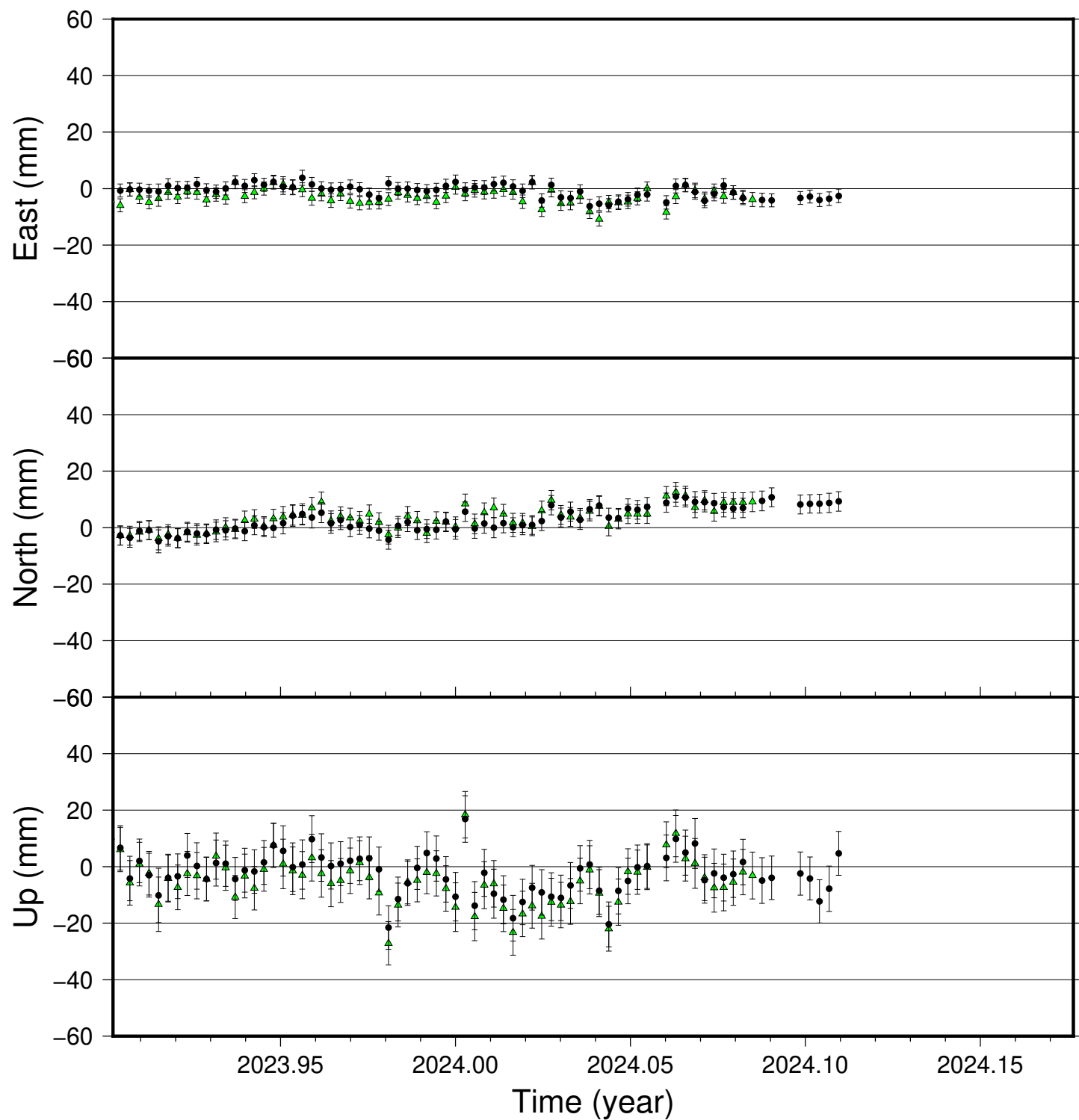
ALM8 time series (IGS 2014), last 100 days
