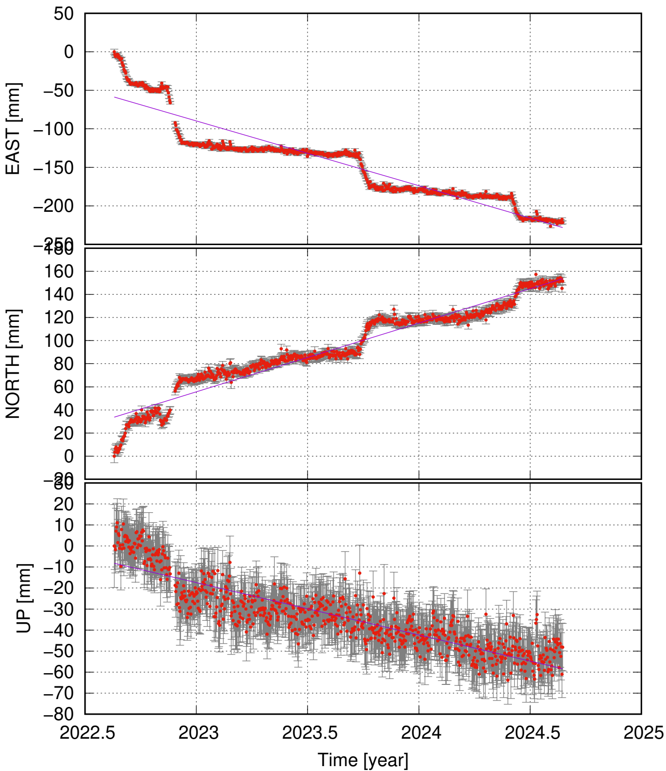
ALM7 (66.15, -19.05) time series (ITRF 2014) v_e = -84.00 \pm 8.90 ; v_n = 59.46 \pm 4.34 ; v_u = -24.88 \pm 3.78 mm/yr
