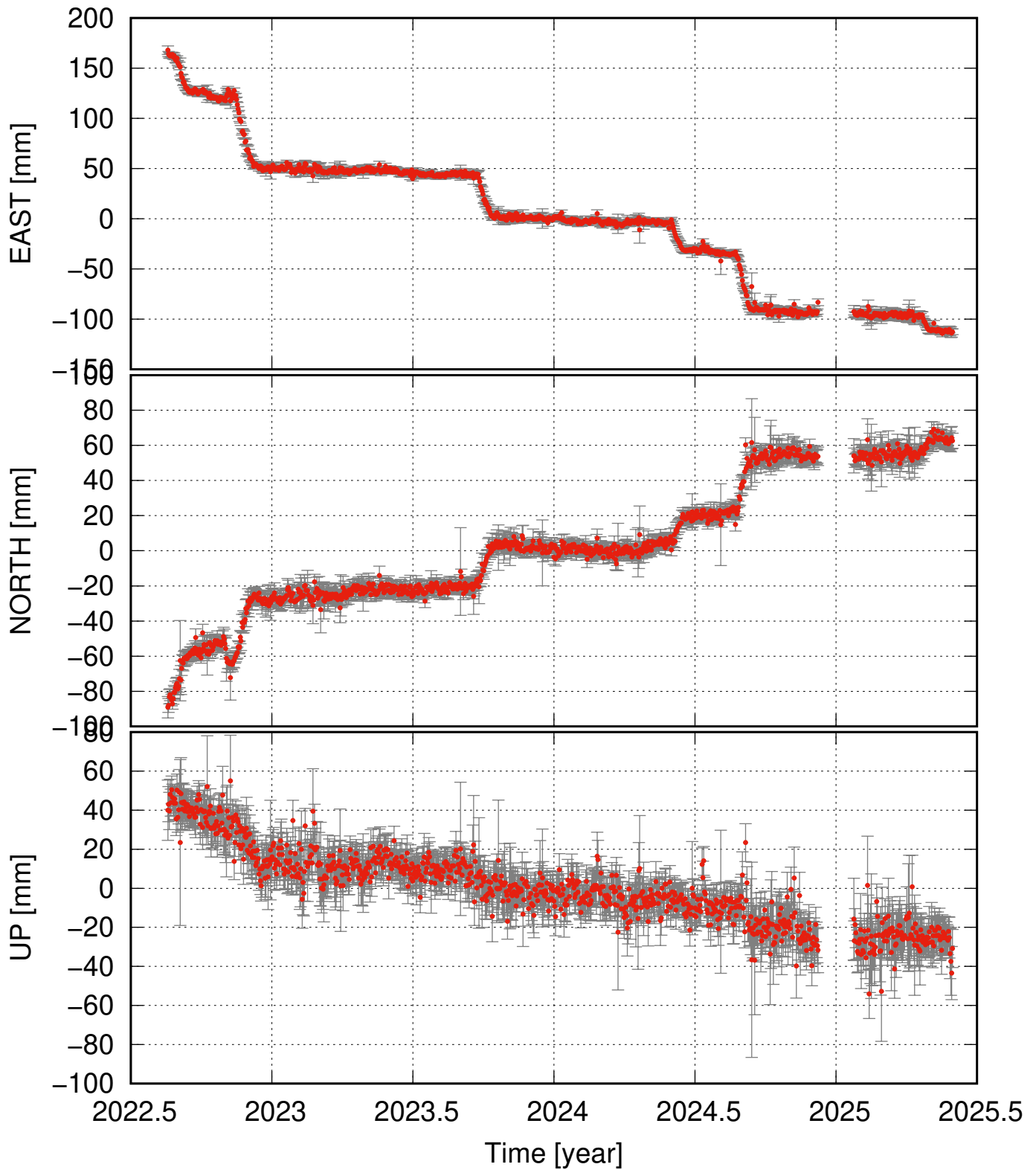
ALM7 time series relative to the NA plate
