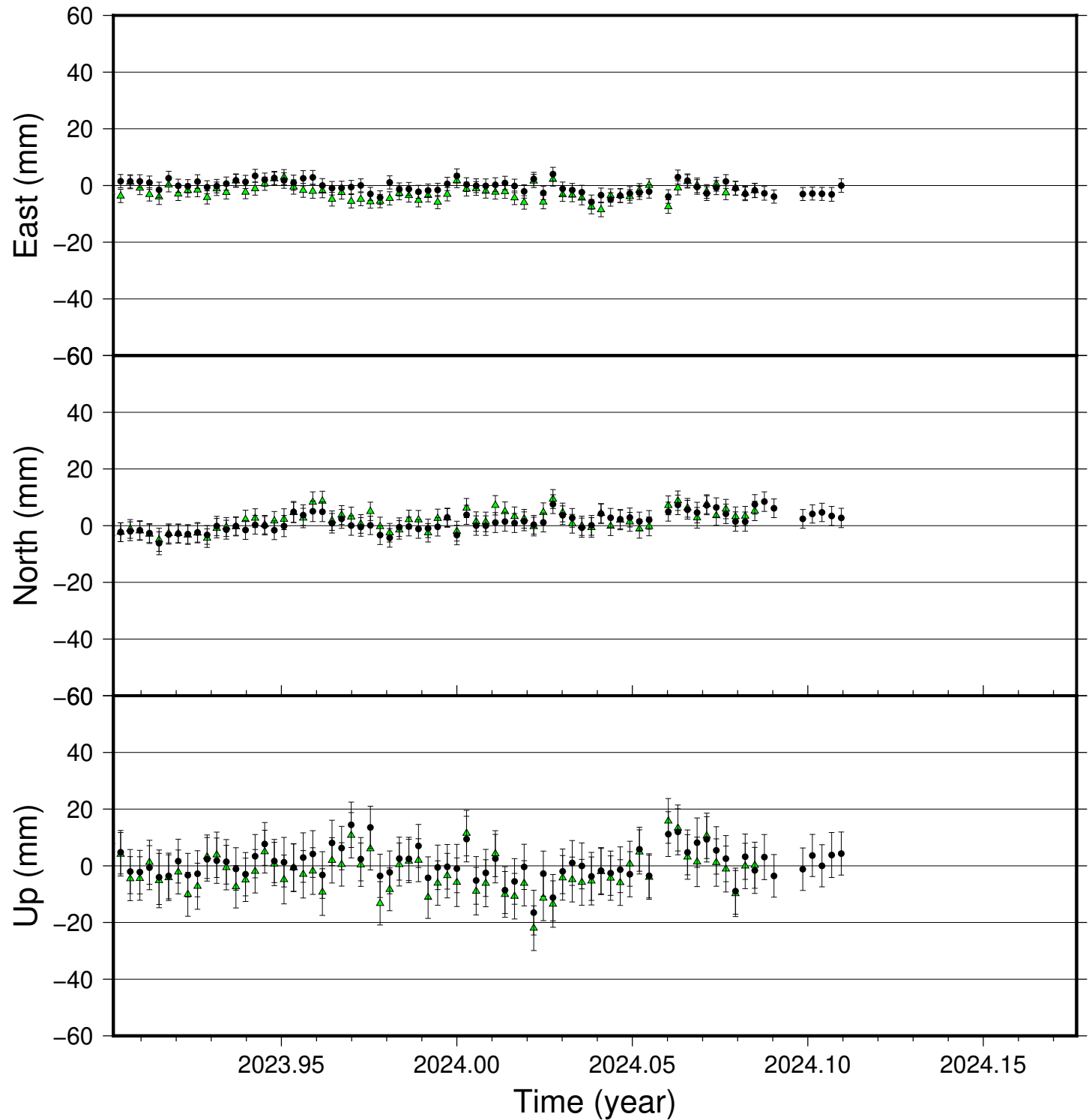
ALM6 time series (IGS 2014), last 100 days
