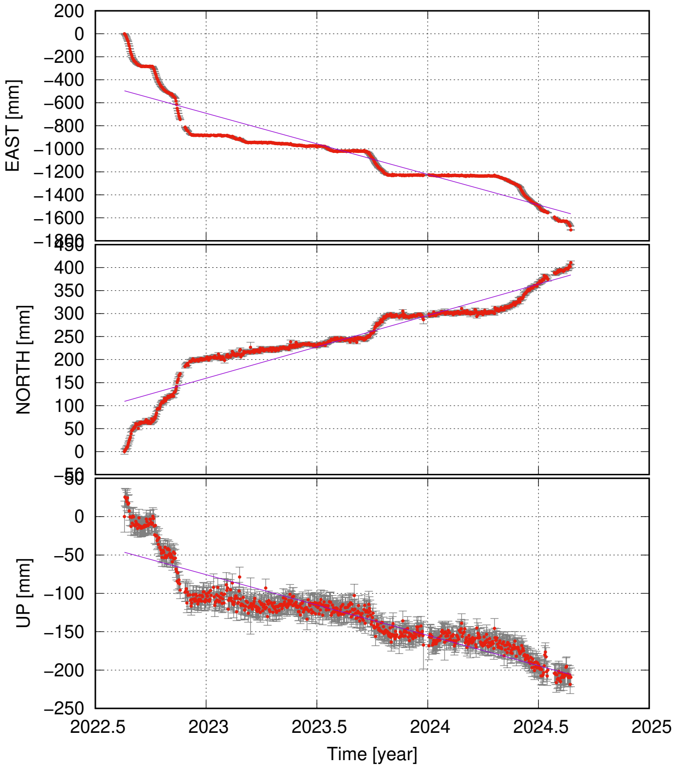
ALM5 (66.15, -19.06) time series (ITRF 2014) v_e = -530.61 \pm 64.71 ; v_n = 136.30 \pm 14.35 ; v_u = -79.07 \pm 10.01 mm/yr
