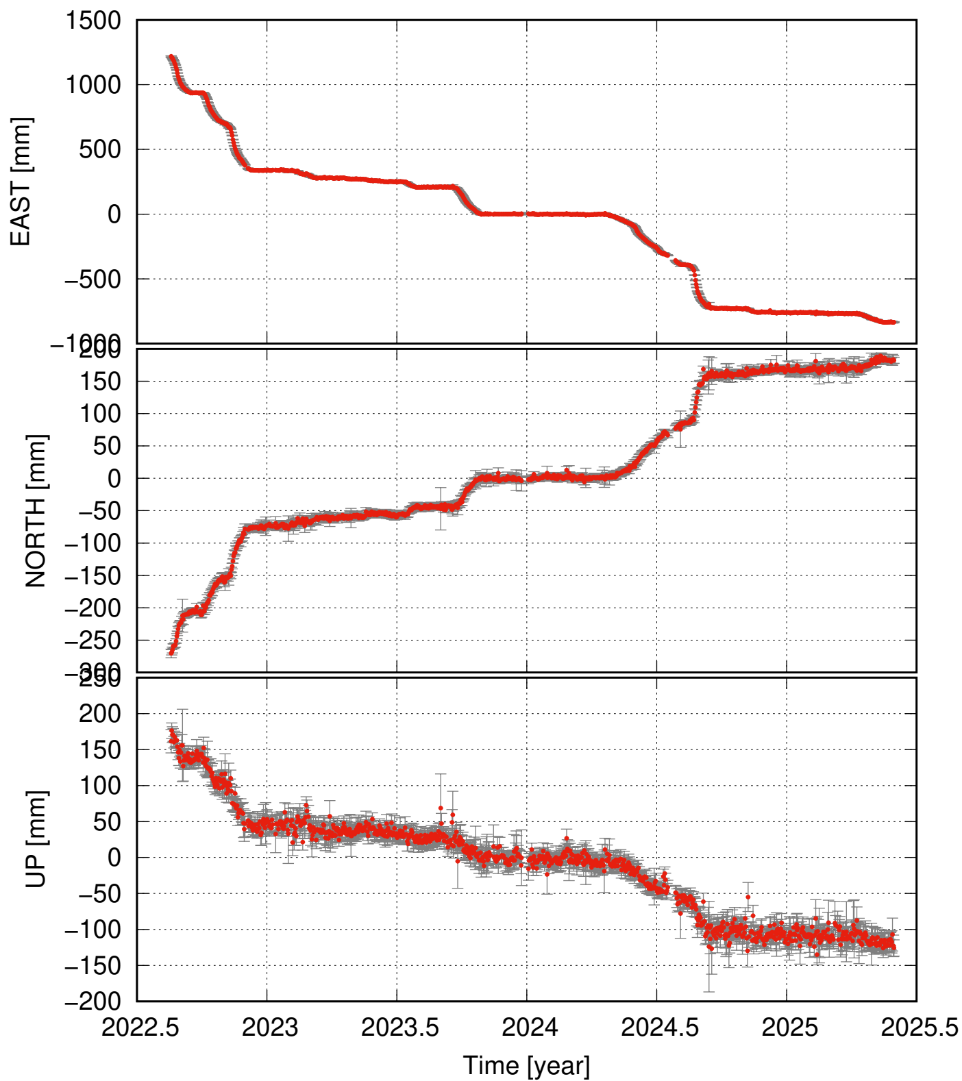
ALM5 time series relative to the NA plate
