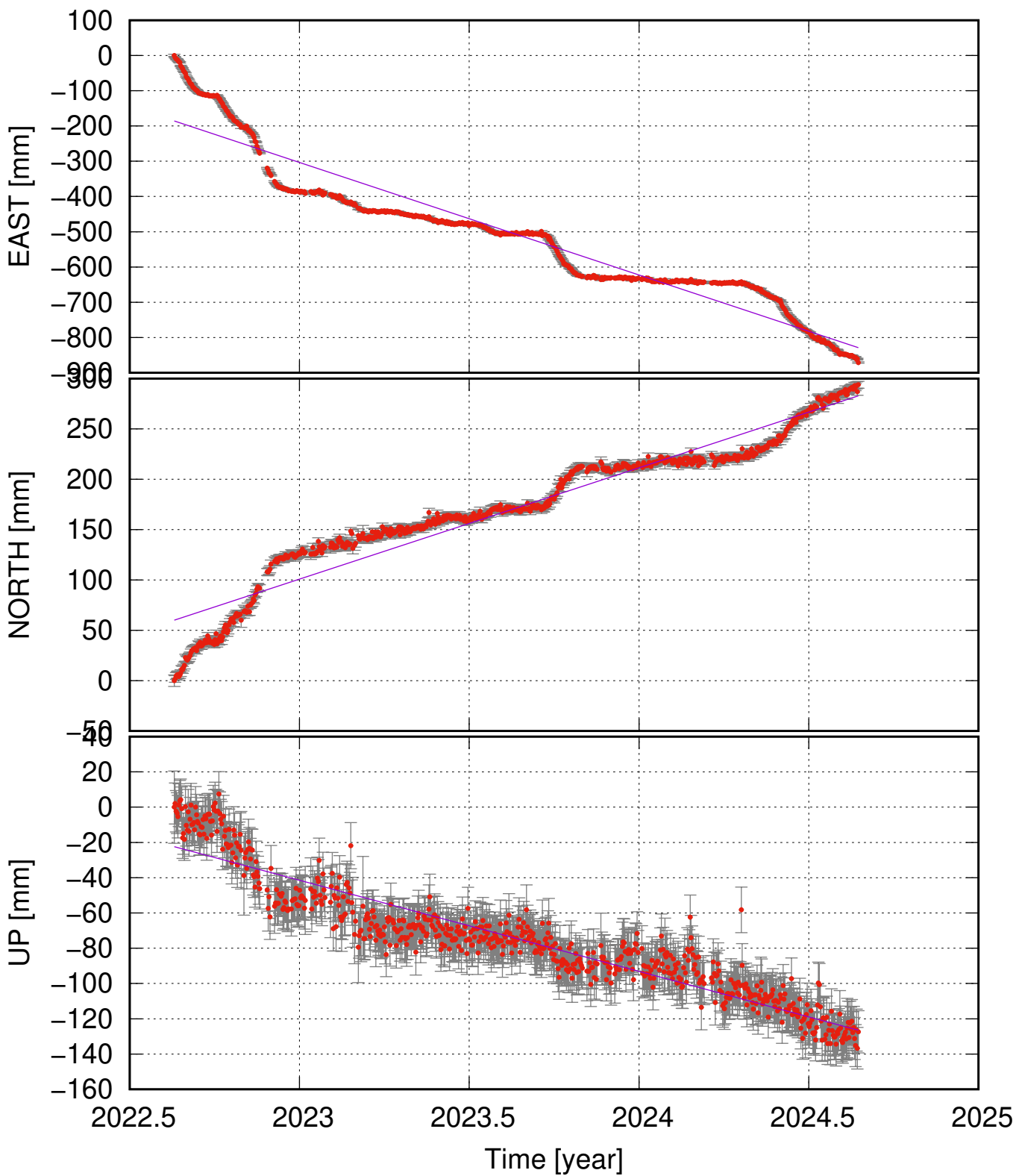
ALM4 (66.15, -19.06) time series (ITRF 2014) v_e = -319.26 \pm 28.15 ; v_n = 110.55 \pm 8.91 ; v_u = -51.60 \pm 5.53 mm/yr
