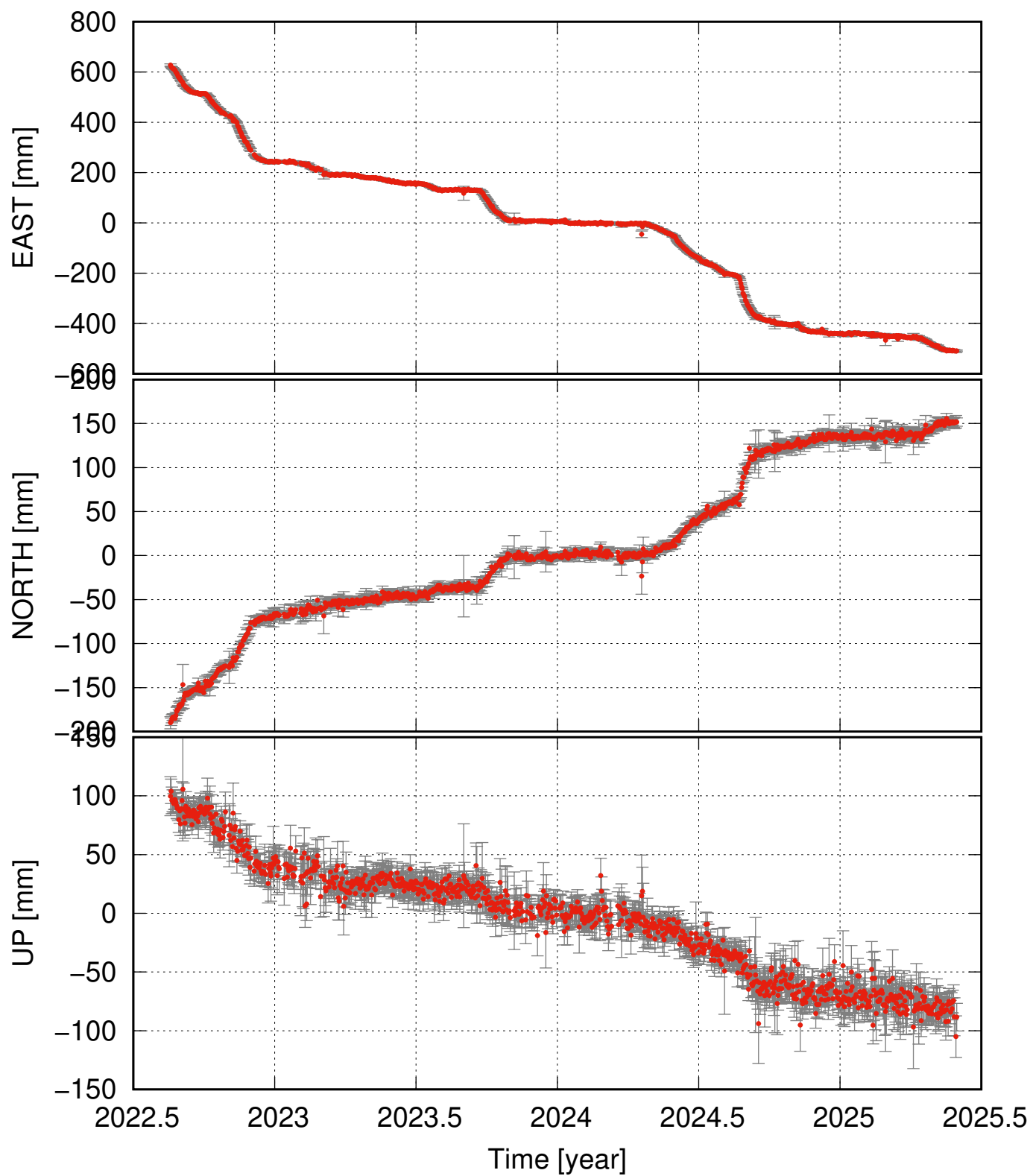
ALM4 time series relative to the NA plate
