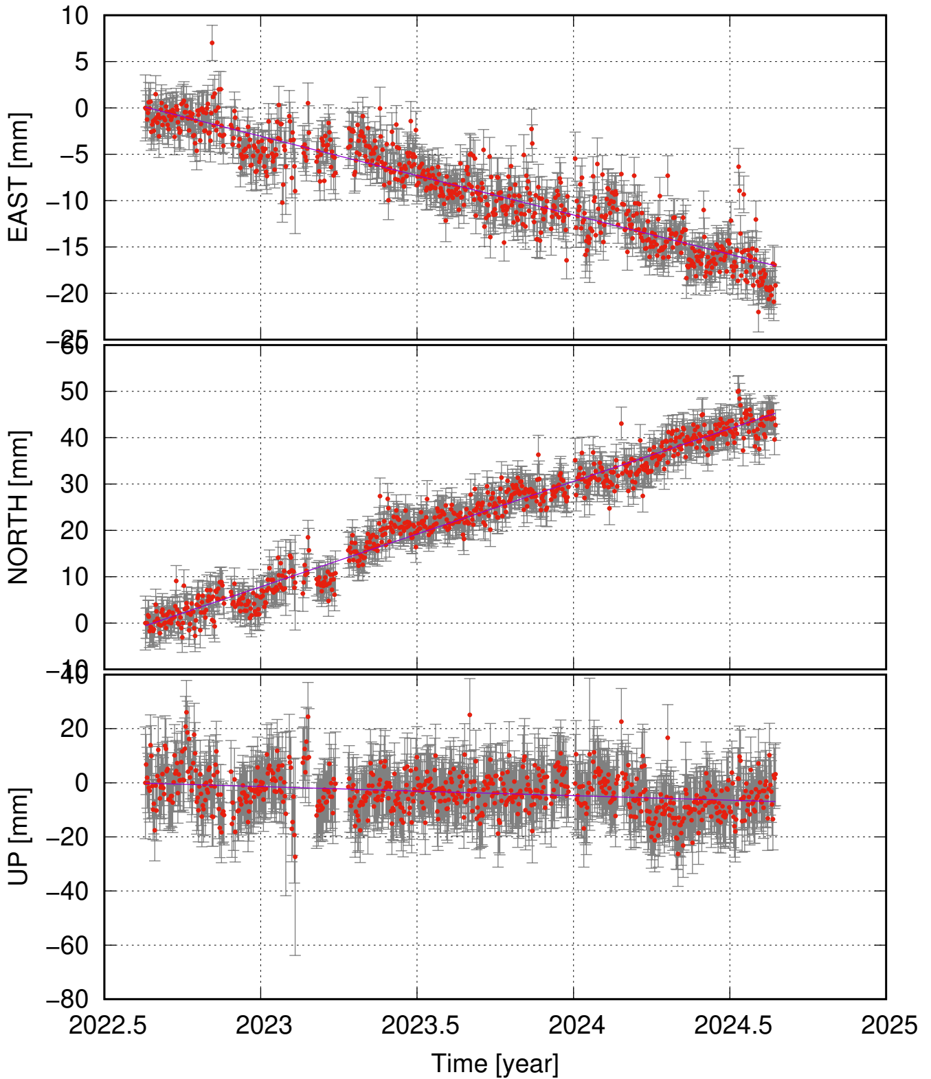
ALM3 (66.14, -19.06) time series (ITRF 2014) v_e = -8.49 \pm 1.05 ; v_n = 22.72 \pm 1.33 ; v_u = -3.36 \pm 3.61 mm/yr
