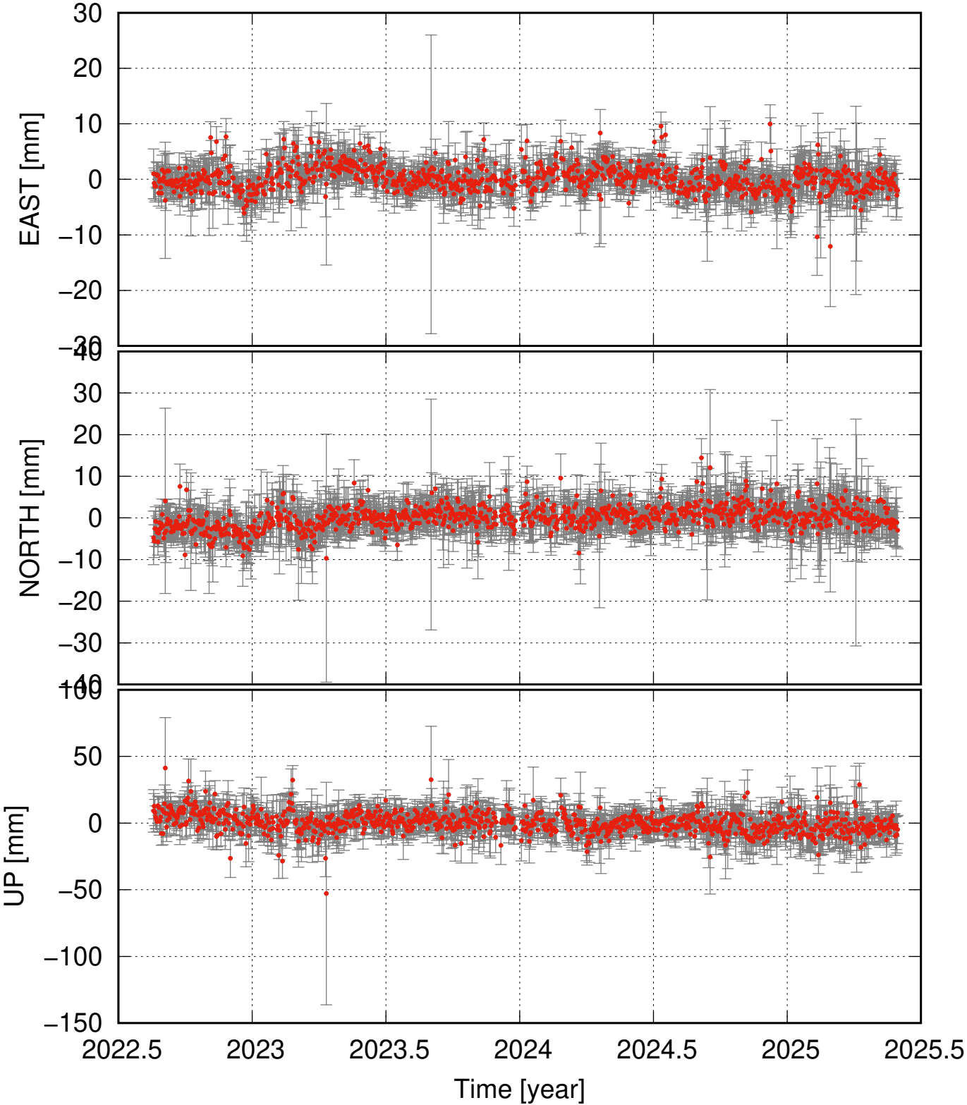
ALM3 time series relative to the NA plate
