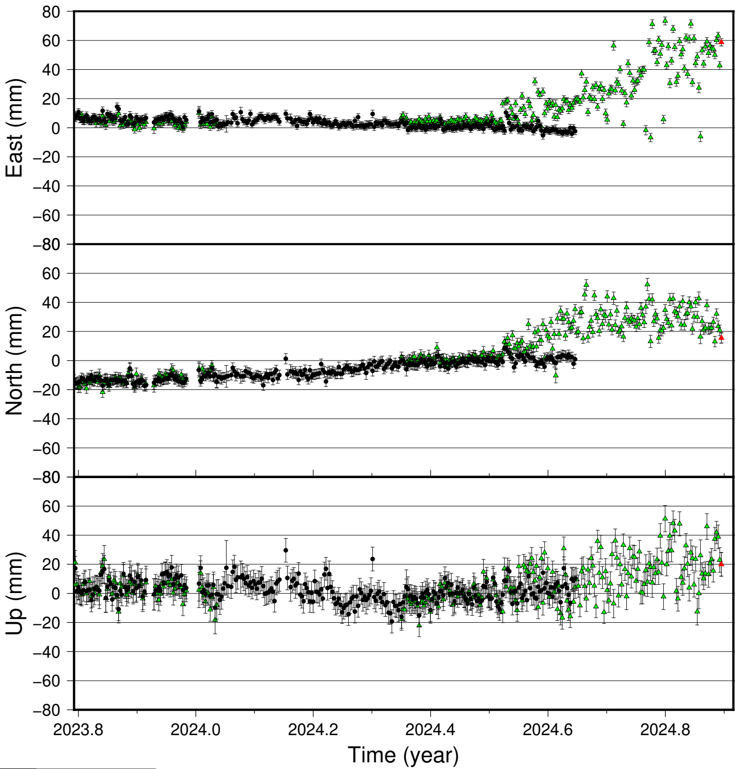
ALM3 time series (IGS 2014), last 400 days
