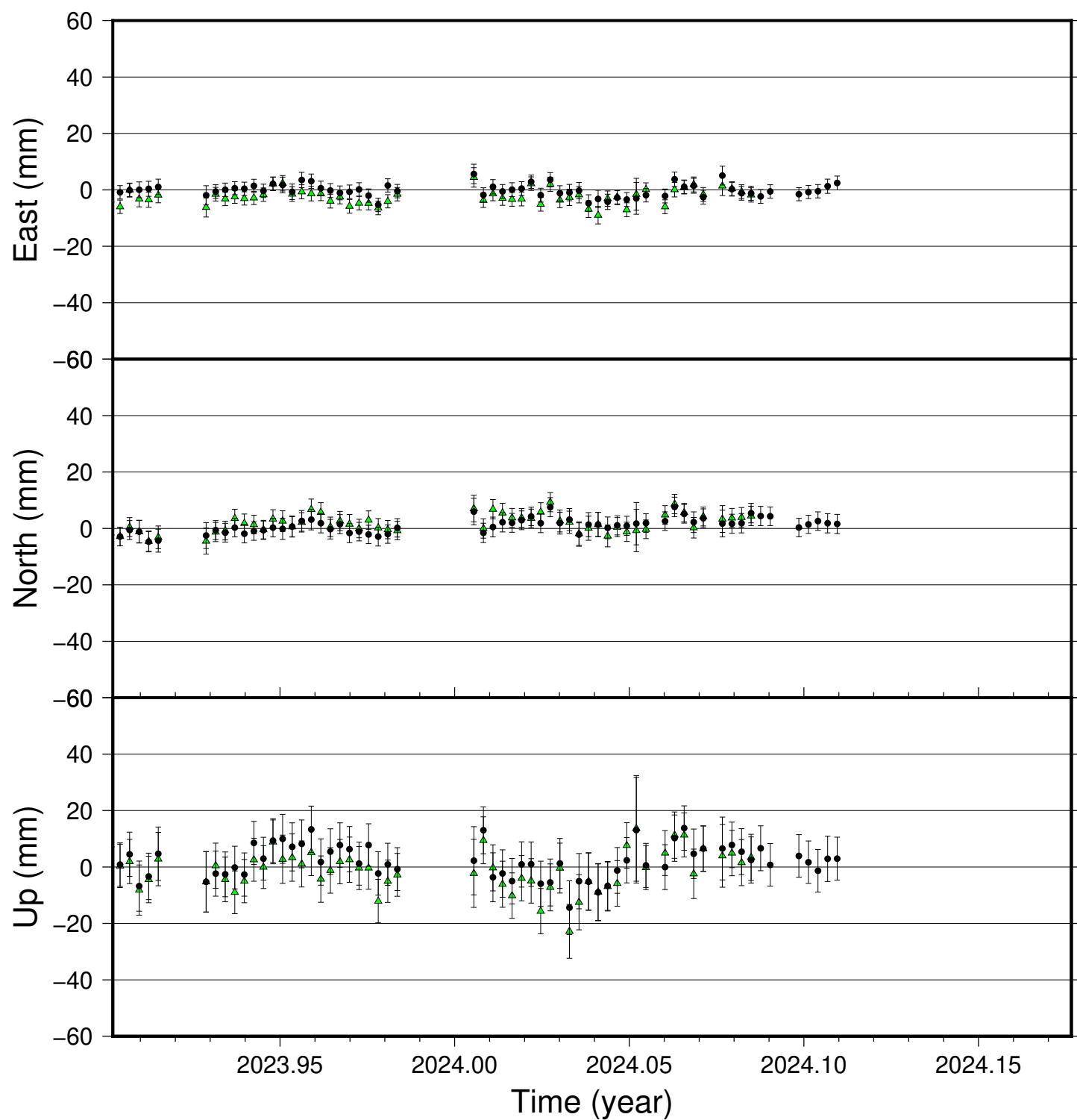
ALM3 time series (IGS 2014), last 100 days
