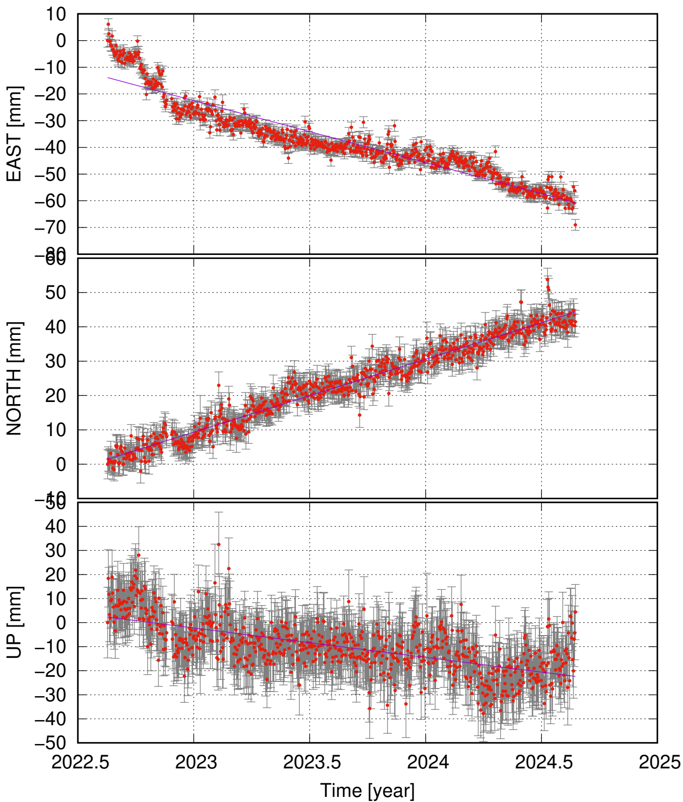
ALM2 (66.13, -19.07) time series (ITRF 2014) v_e = -23.19 \pm 2.37 ; v_n = 21.24 \pm 1.29 ; v_u = -12.22 \pm 4.08 mm/yr
