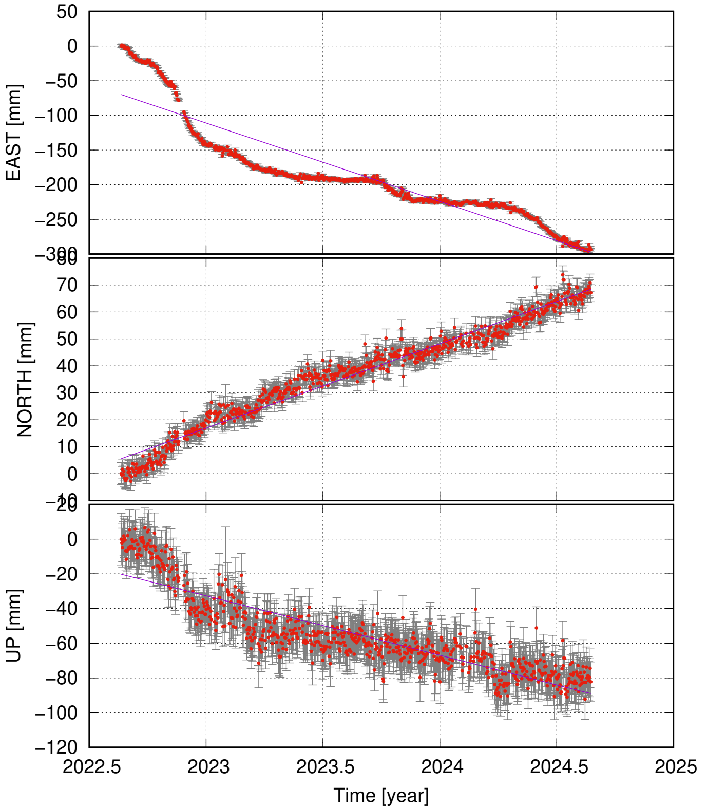
ALM1 (66.11, -19.07) time series (ITRF 2014) v_e = -113.06 \pm 14.15 ; v_n = 31.28 \pm 1.79 ; v_u = -34.23 \pm 5.31 mm/yr
