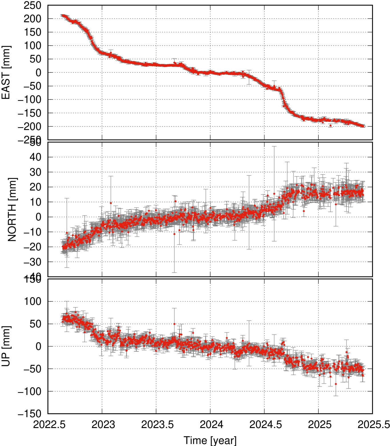
ALM1 time series relative to the NA plate
