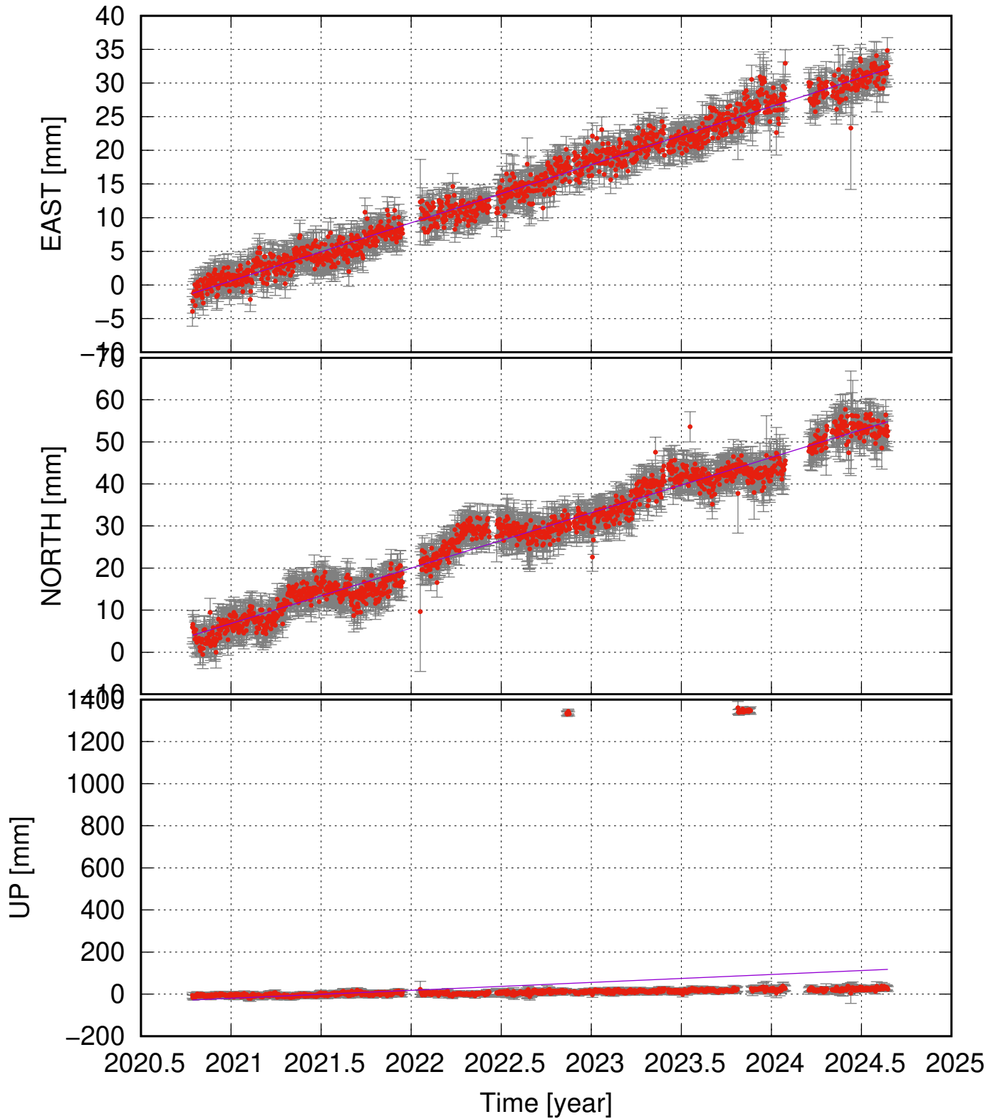
ALHV (63.45, -18.31) time series (ITRF 2014) v_e = 8.64 \pm 0.36 ; v_n = 13.16 \pm 0.68 ; v_u = 37.71 \pm 53.97 mm/yr
