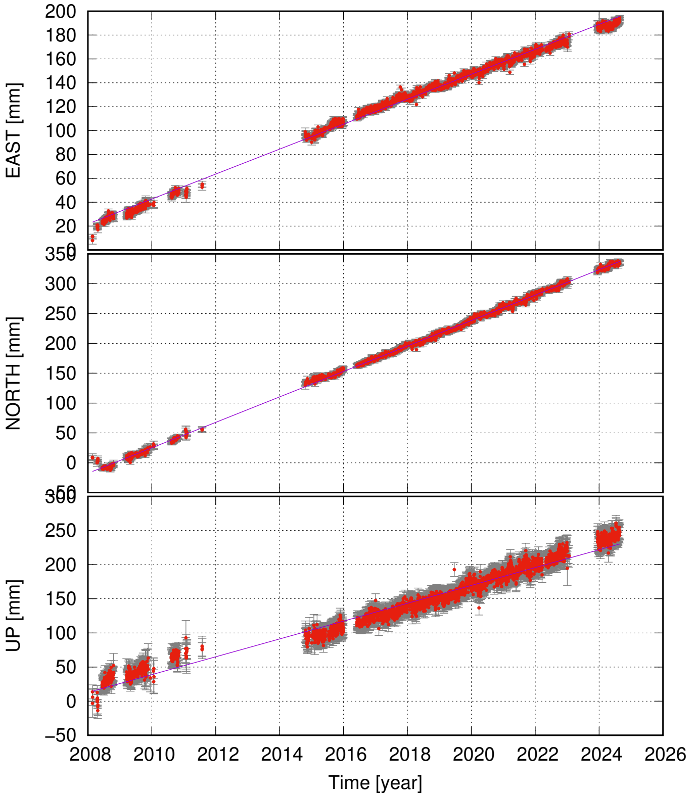
ALFD (64.98, -16.03) time series (ITRF 2014) v_e = 10.45 \pm 0.18 ; v_n = 21.33 \pm 0.18 ; v_u = 13.06 \pm 0.60 mm/yr
