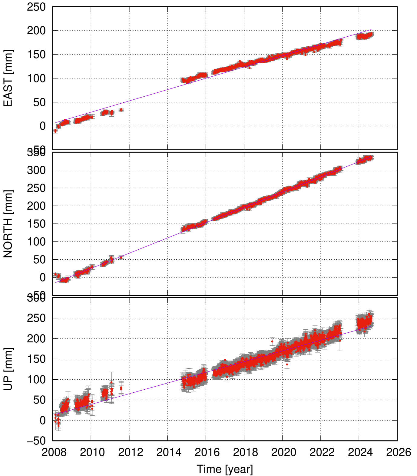
ALFD (64.98, -16.03) time series (ITRF 2014) ve = 11.83 ± 0.39; vn = 21.33 ± 0.18; vu = 13.06 ± 0.60 mm/yr
