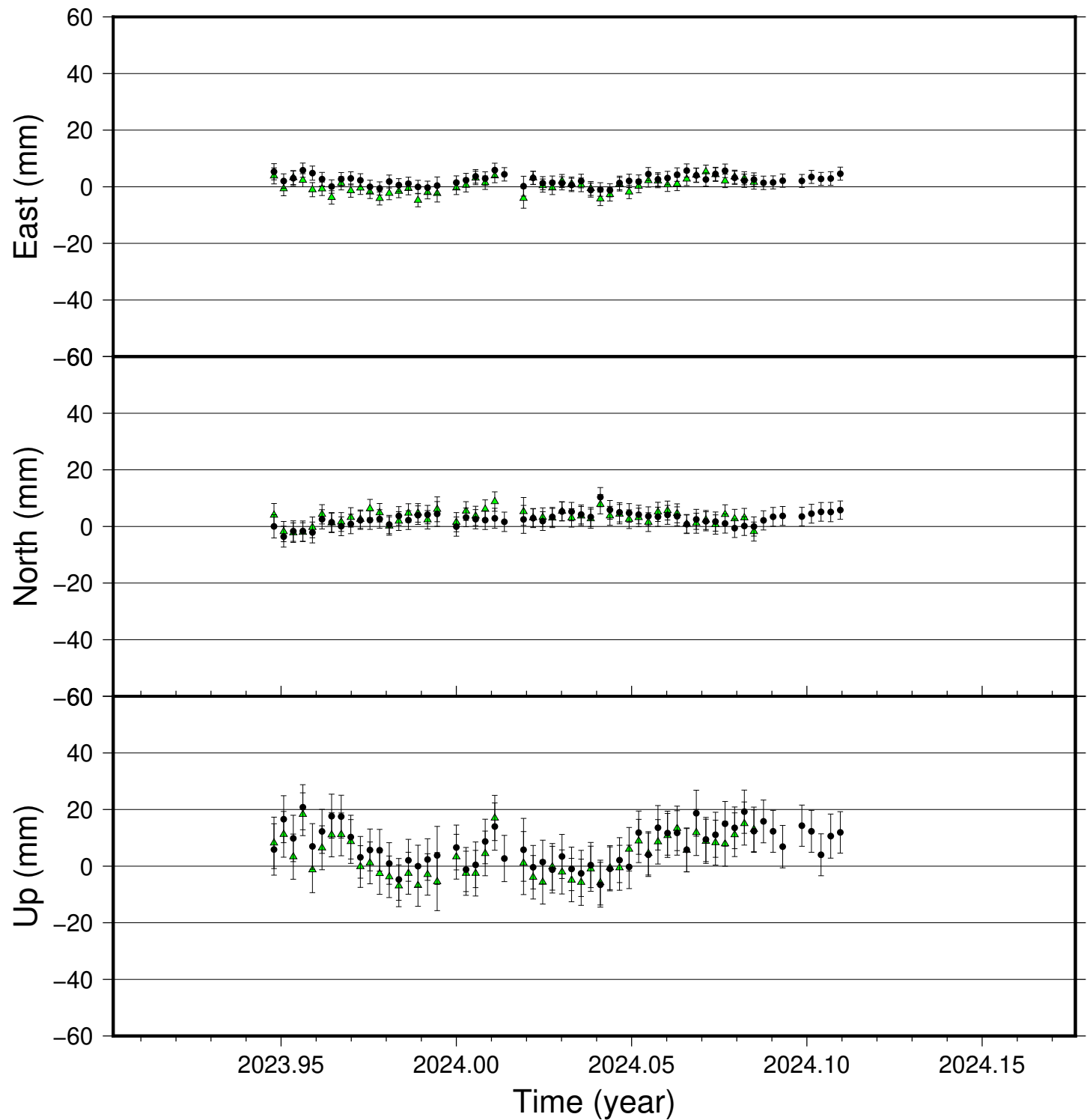
ALFD time series (IGS 2014), last 100 days
