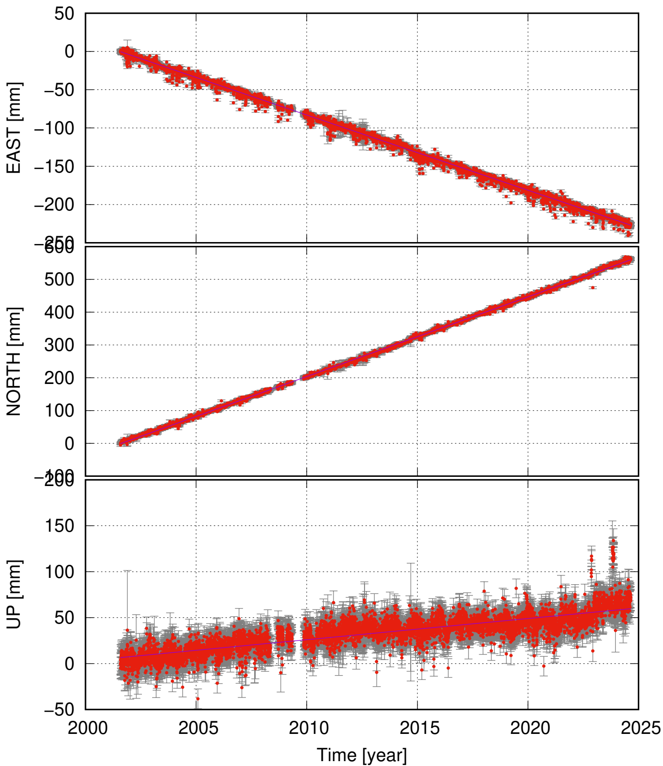
AKUR (65.69, -18.12) time series (ITRF 2014) v_e = -9.83 \pm 0.13 ; v_n = 24.30 \pm 0.14 ; v_u = 2.31 \pm 0.42 mm/yr
