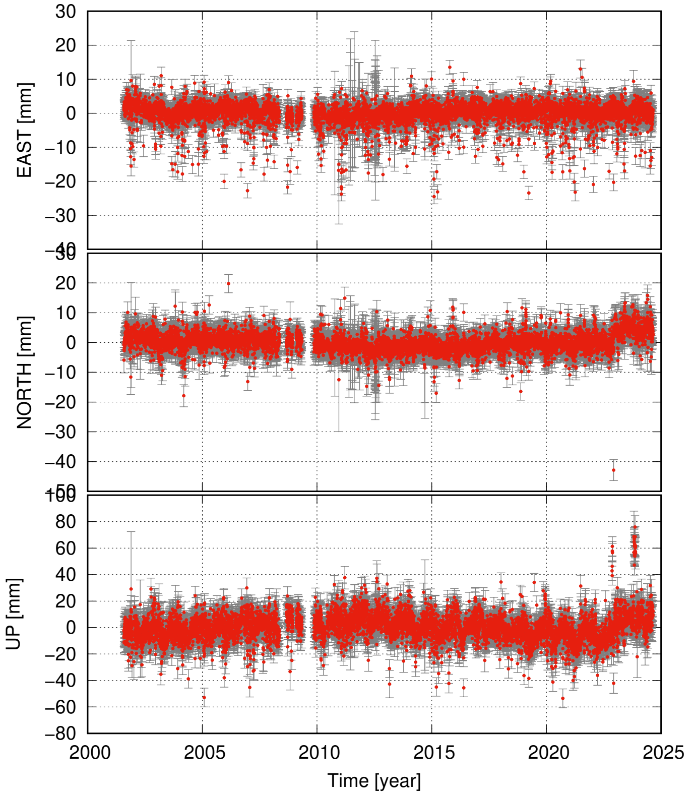
AKUR residual time series (some major events removed as well)
