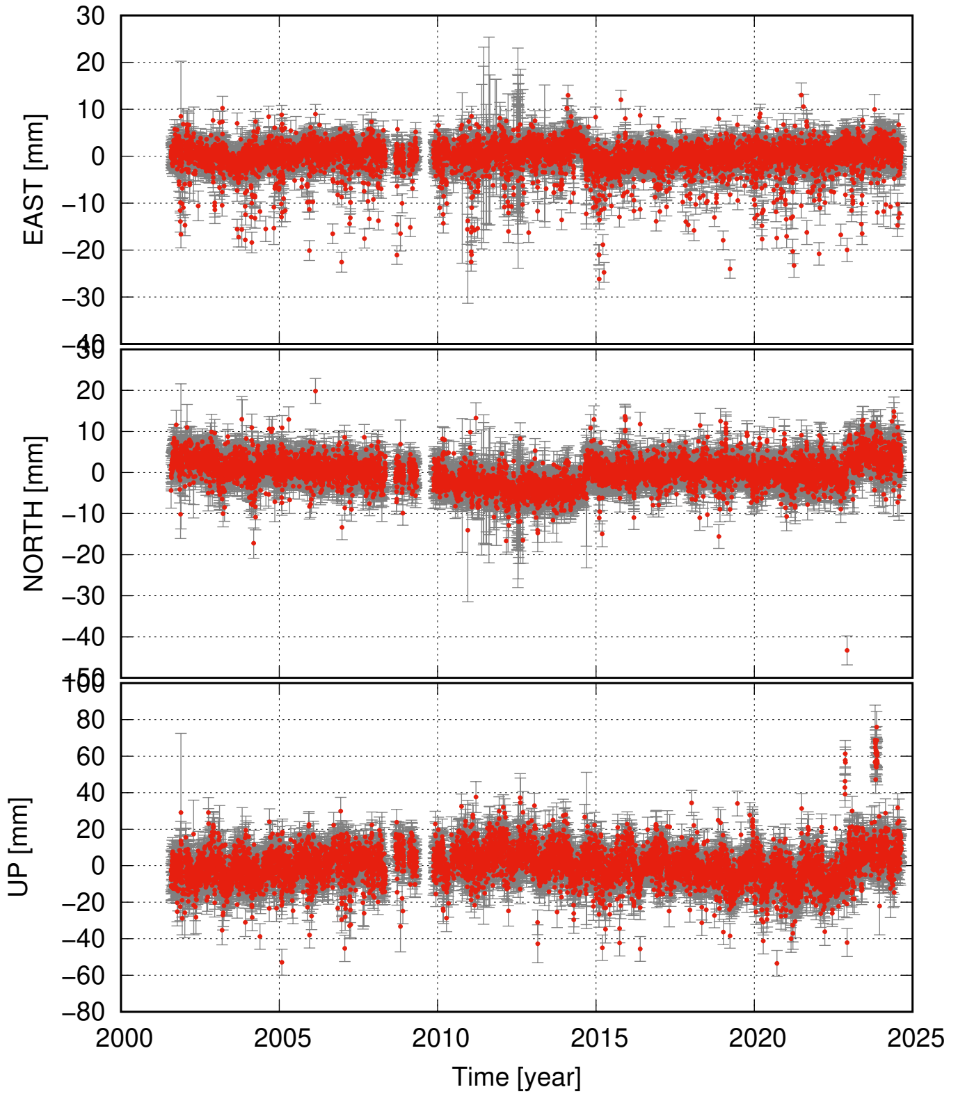
AKUR residual time series
