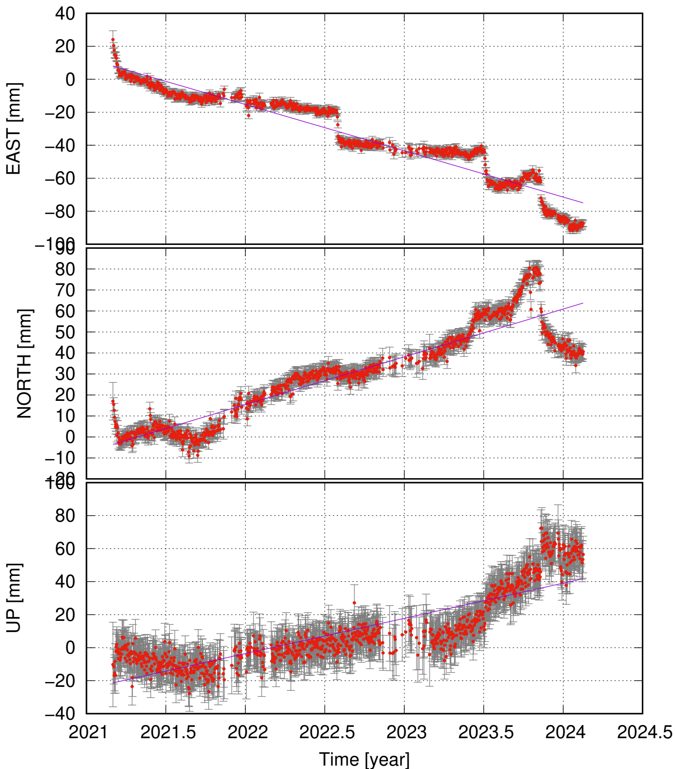
AFST (63.98, -22.14) time series (ITRF 2014) v_e = -28.04 \pm 2.48 ; v_n = 22.74 \pm 2.95 ; v_u = 21.32 \pm 3.88 mm/yr
