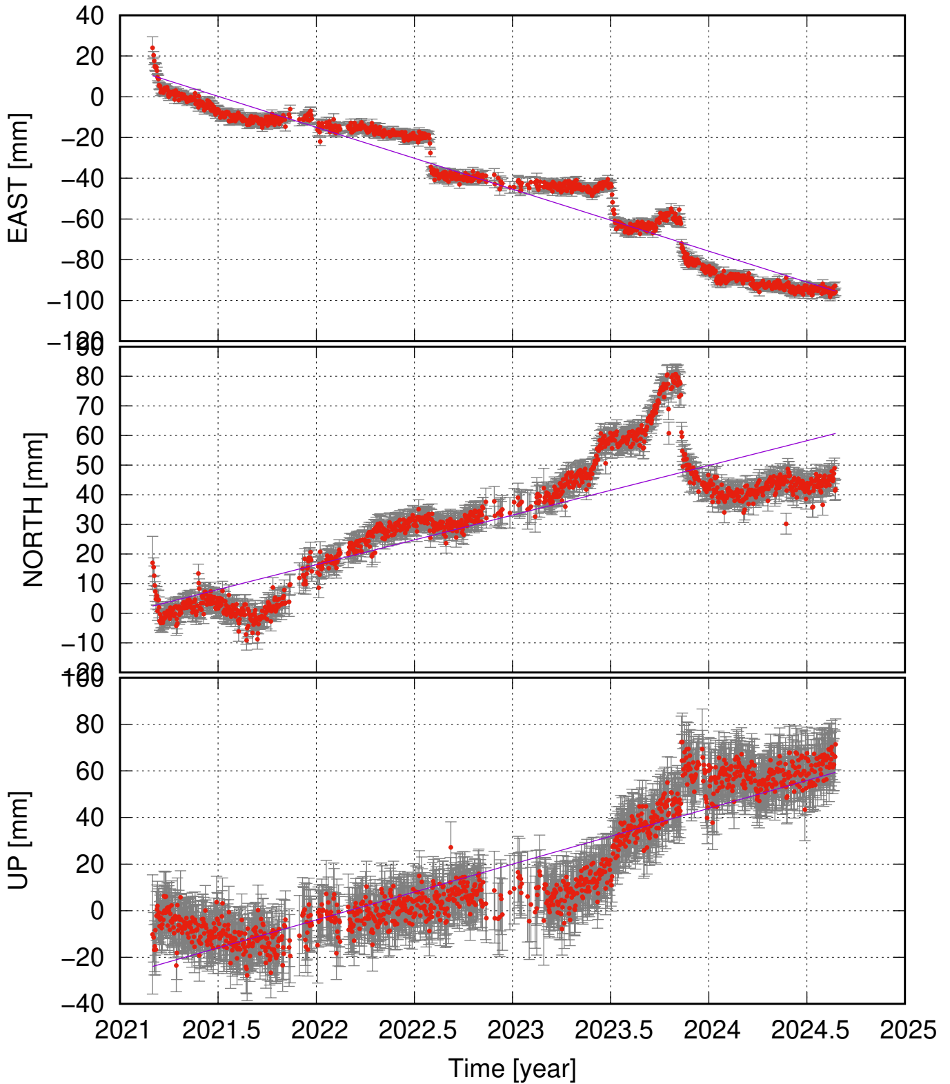
AFST (63.98, -22.14) time series (ITRF 2014) v_e = -30.40 \pm 2.14 ; v_n = 16.73 \pm 3.24 ; v_u = 23.95 \pm 3.21 mm/yr
